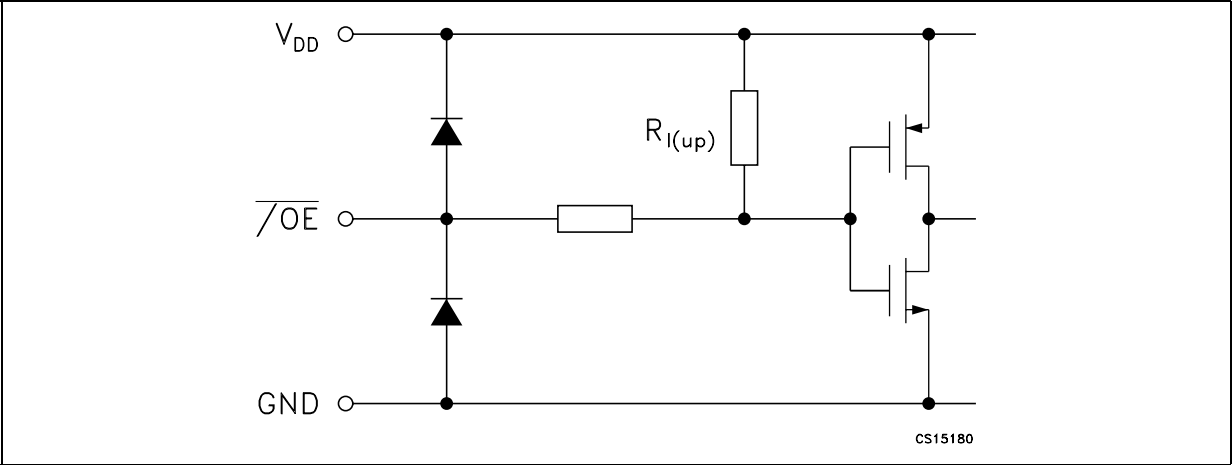
Figure 2: \overline{OE} Terminal
